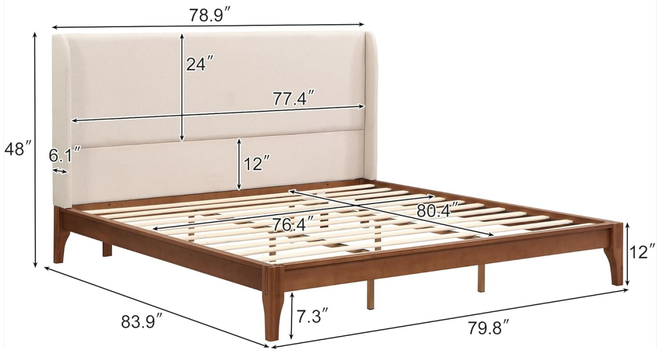
Image 8.1: Detailed dimensions for the King size platform bed frame.
