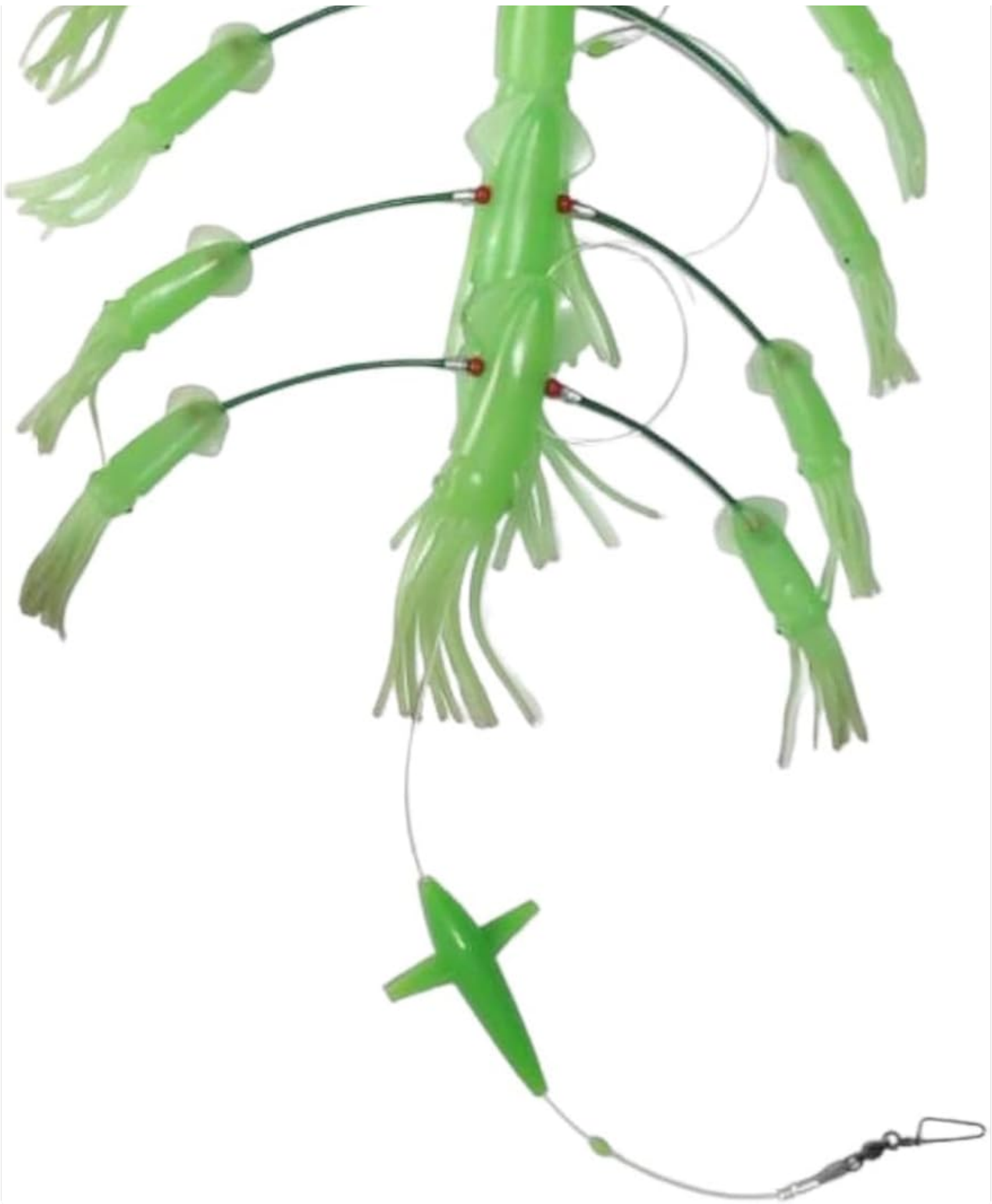
Figure 2.4: The Masterpro Flippy Floppy Offshore Squid Teaser in its complete assembly.
