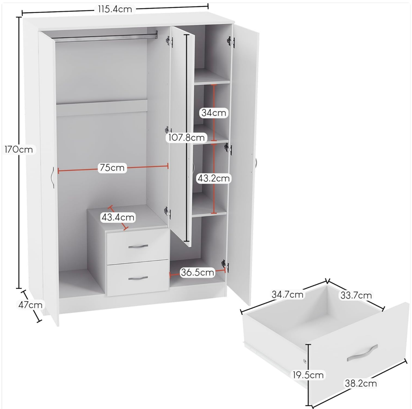
Image: A detailed diagram illustrating the precise dimensions of the Vida Designs Riano wardrobe, including its height, width, and depth, along with internal measurements for shelves and hanging space.
