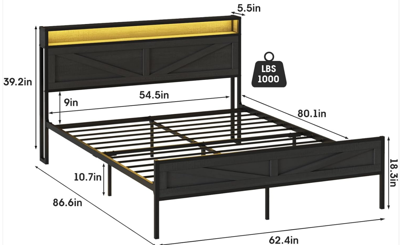
Figure 4.1: Queen Size Bed Frame Dimensions. Overall dimensions are 86.6 inches (L) x 62.4 inches (W) x 39.2 inches (H). The headboard is 39.2 inches high, and the footboard is 18.3 inches high. Under-bed clearance is 10.7 inches.
