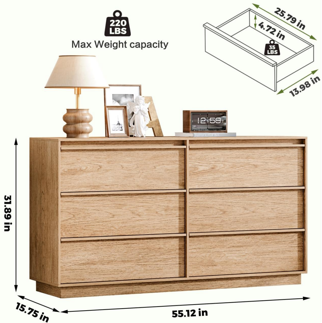
Image 5.2: An image detailing the overall dimensions of the chest (15.75"D x 55.12"W x 31.9"H), the maximum weight capacity for the top surface (220 lbs), and for each drawer (35 lbs).
