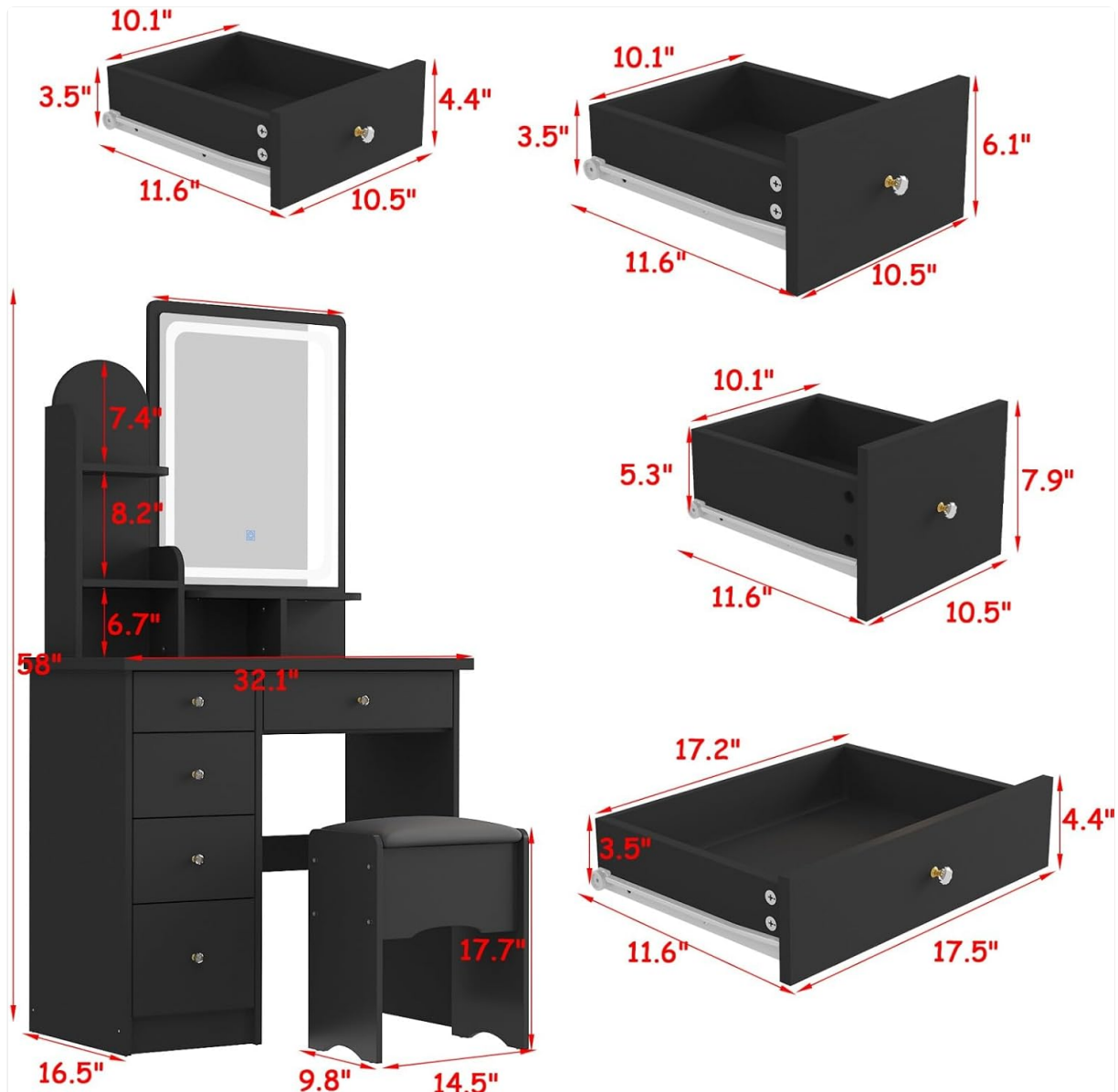
Figure 3: Detailed dimensions of the vanity set components, useful for planning placement and assembly.
