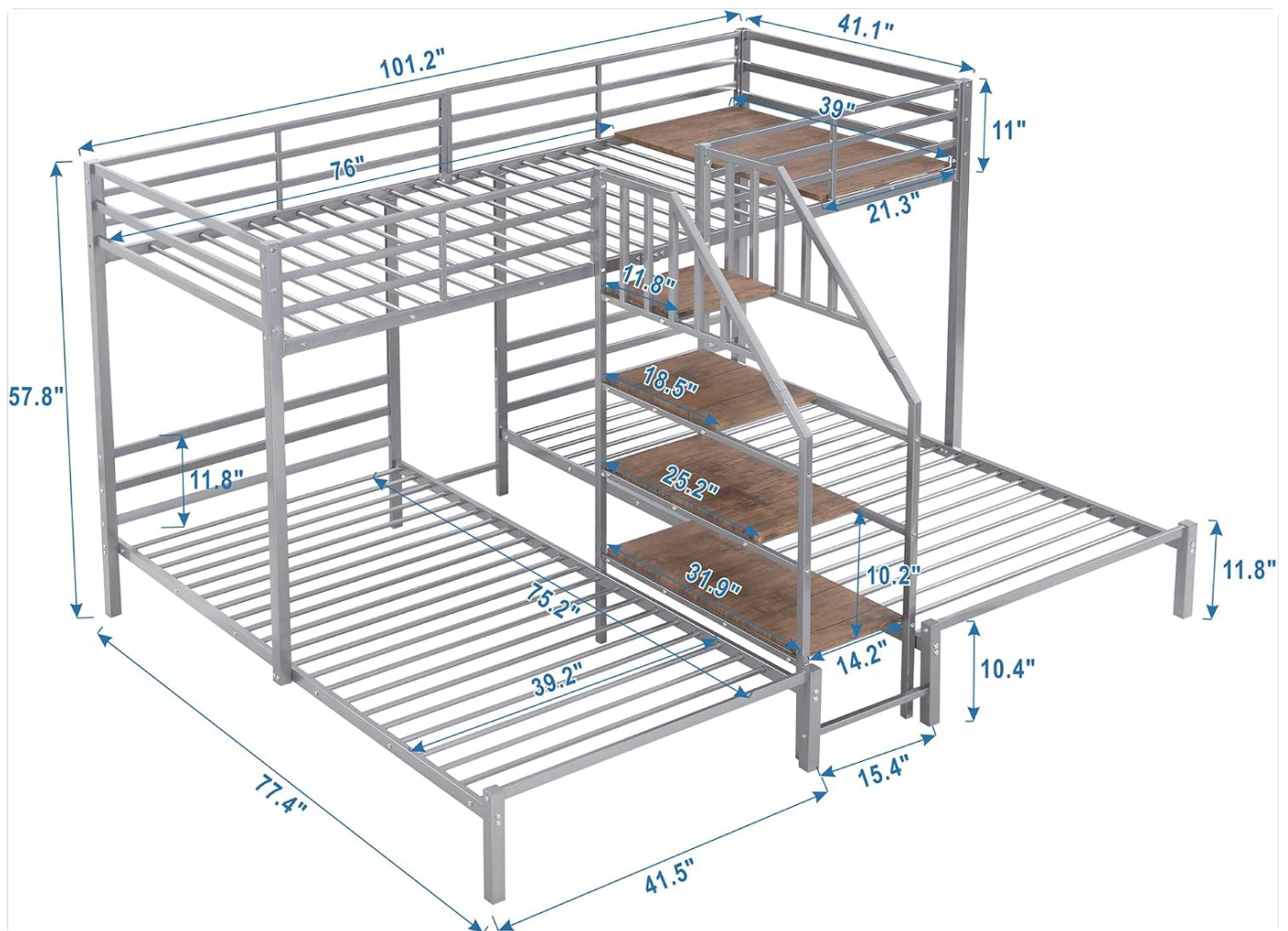
Image: A detailed diagram showing the dimensions of the SOFTSEA Triple Metal Bunk Bed, including length, width, and height measurements.
