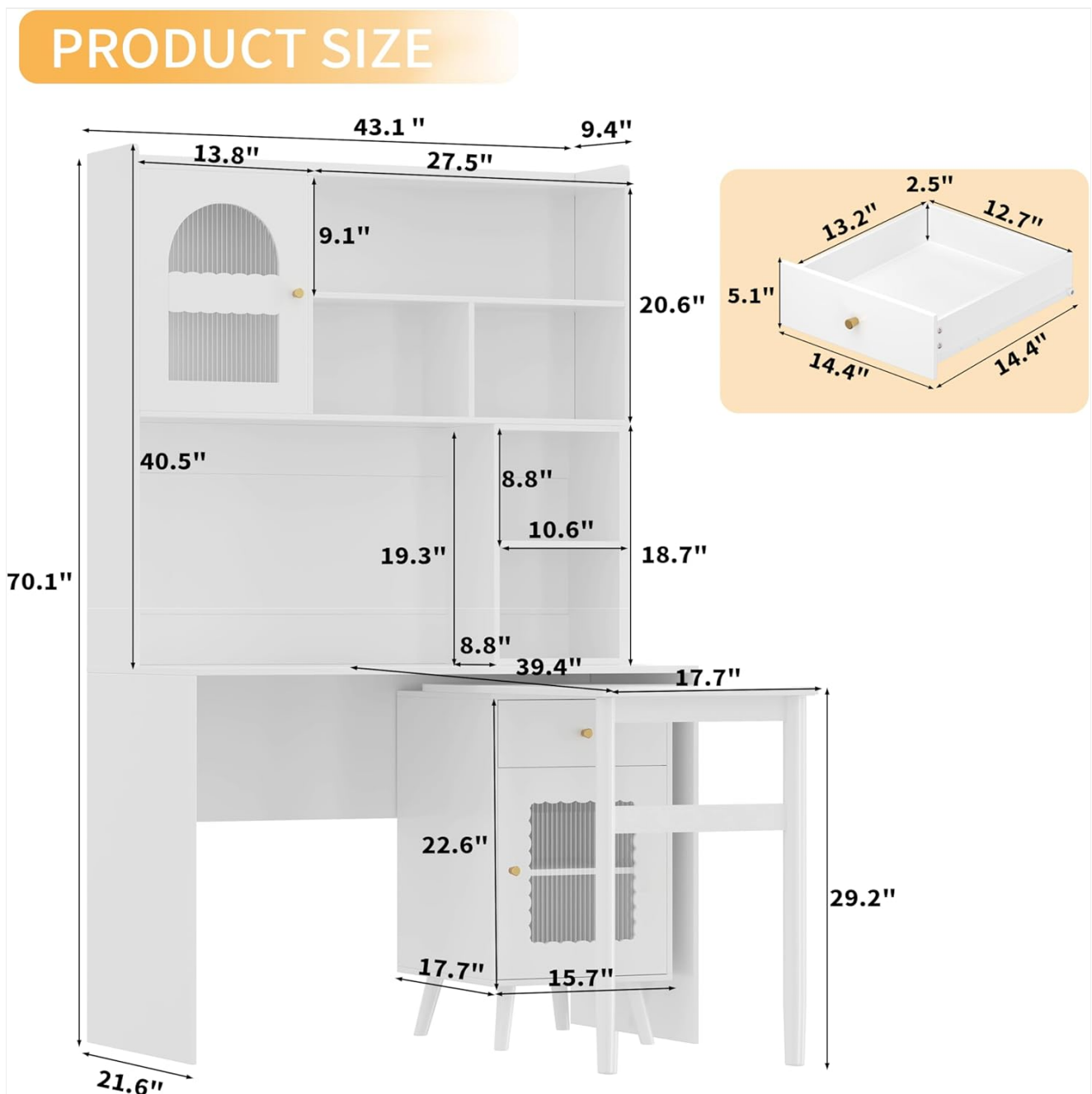
Image 3.1: Product dimensions for the Merax Computer Desk, including the main body and rotating desktop.
