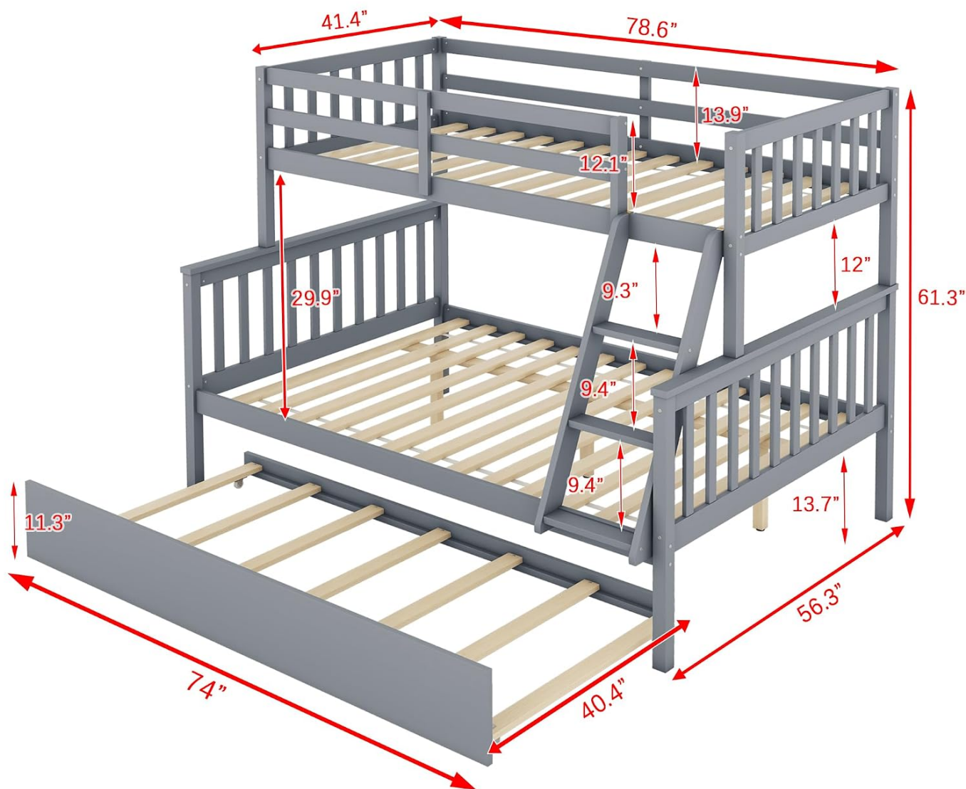
Image 5: A detailed diagram illustrating the dimensions of the LINKHOO Twin Over Full Bunk Bed, including length, width, height, and specific measurements for each bunk and the trundle unit.
