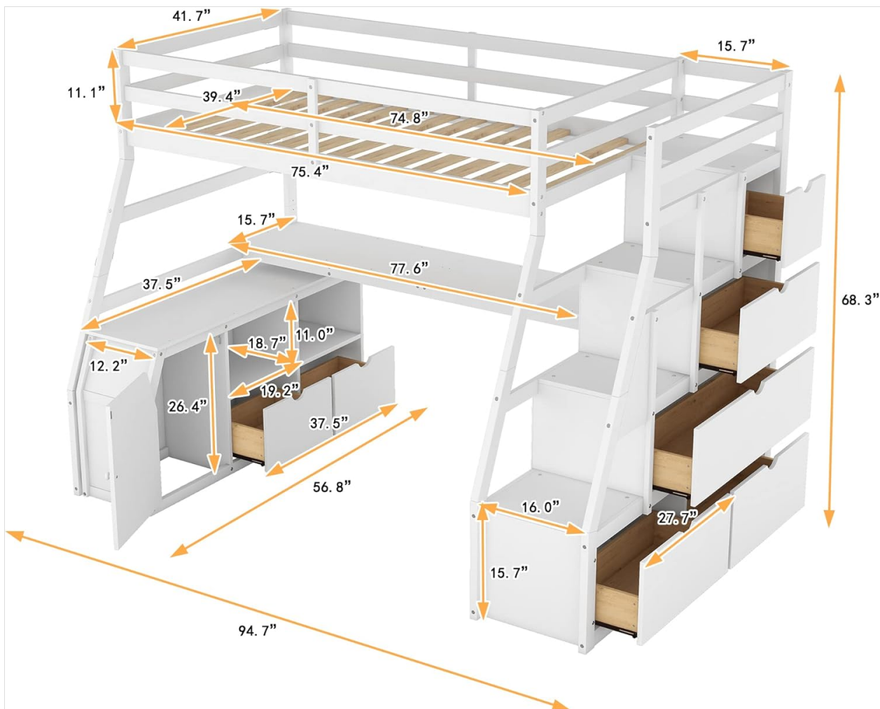
Image: Dimensional diagram of the loft bed, showing overall and component measurements.
