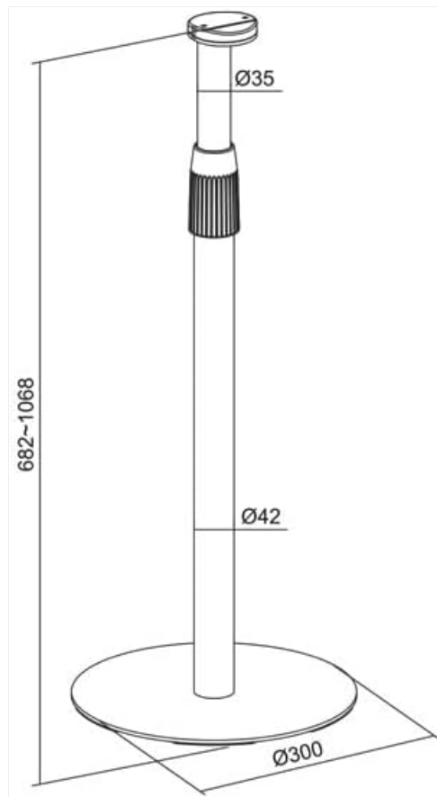
Image: Technical diagram illustrating the dimensions of the speaker stand, including height and base diameter.
