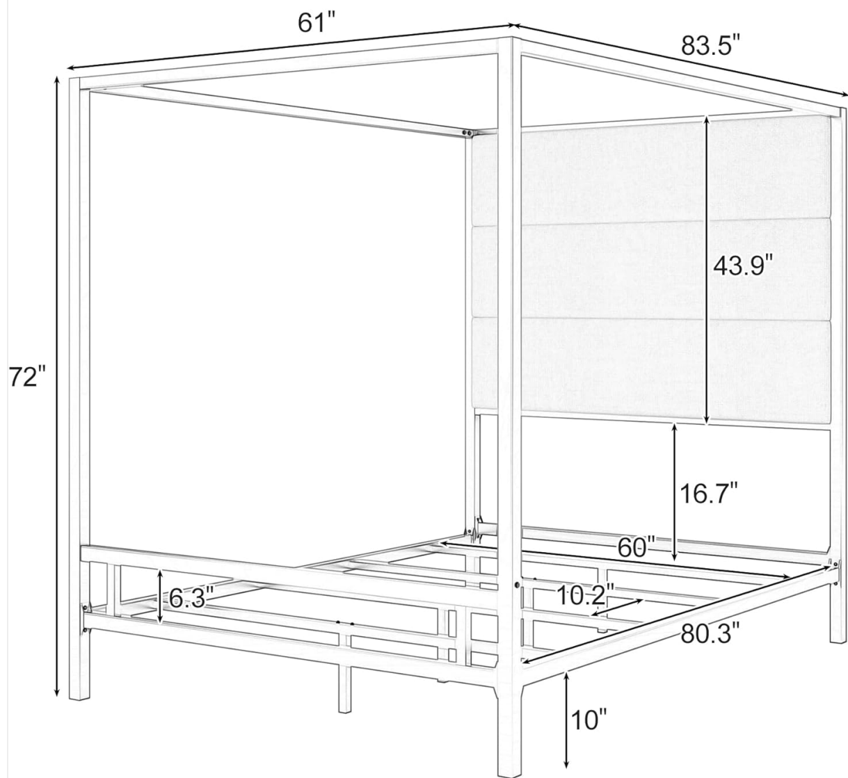
Image: Detailed dimension diagram for the Queen size canopy bed, showing length, width, and height measurements.
