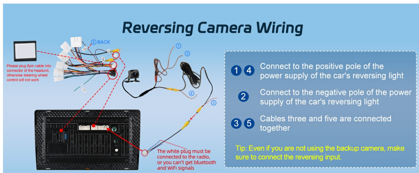
Image: A detailed wiring diagram illustrating how to connect the backup camera to the car stereo and the vehicle's reversing light circuit.
