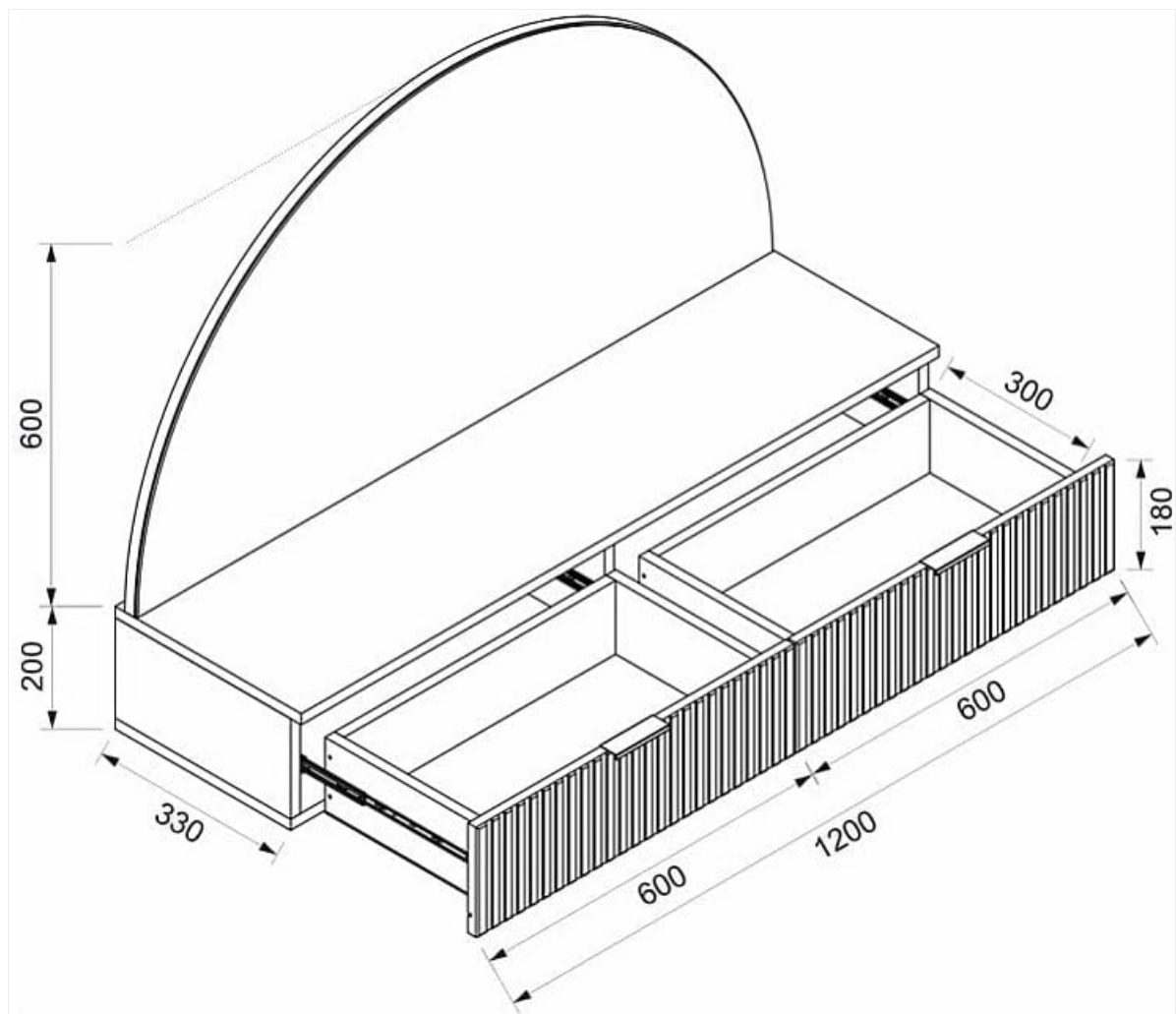
Image 4.1: Assembly diagram showing dimensions and drawer structure.
