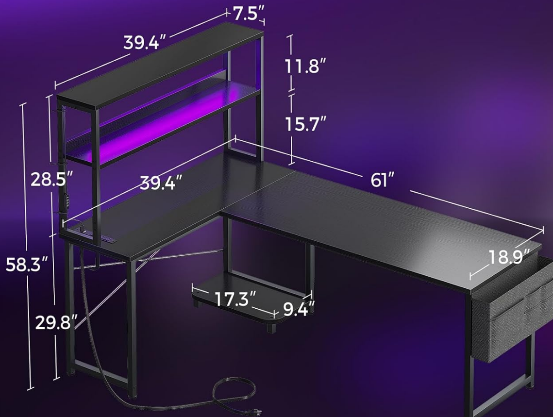
Image: A detailed diagram outlining the specific measurements of the desk, including the main surface, L-extension, and hutch.
