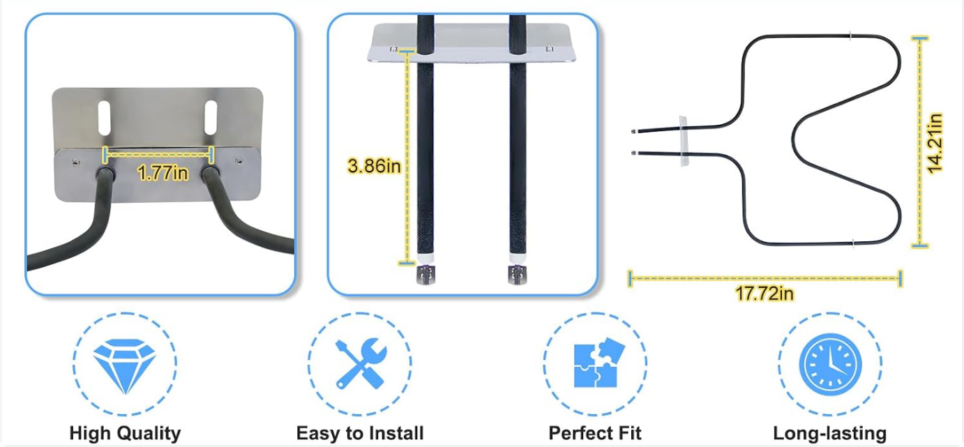
Image: Detailed product dimensions of the heating element, showing a width of 17.72 inches and a height of 14.21 inches, with terminal spacing of 1.77 inches and terminal length of 3.86 inches.
