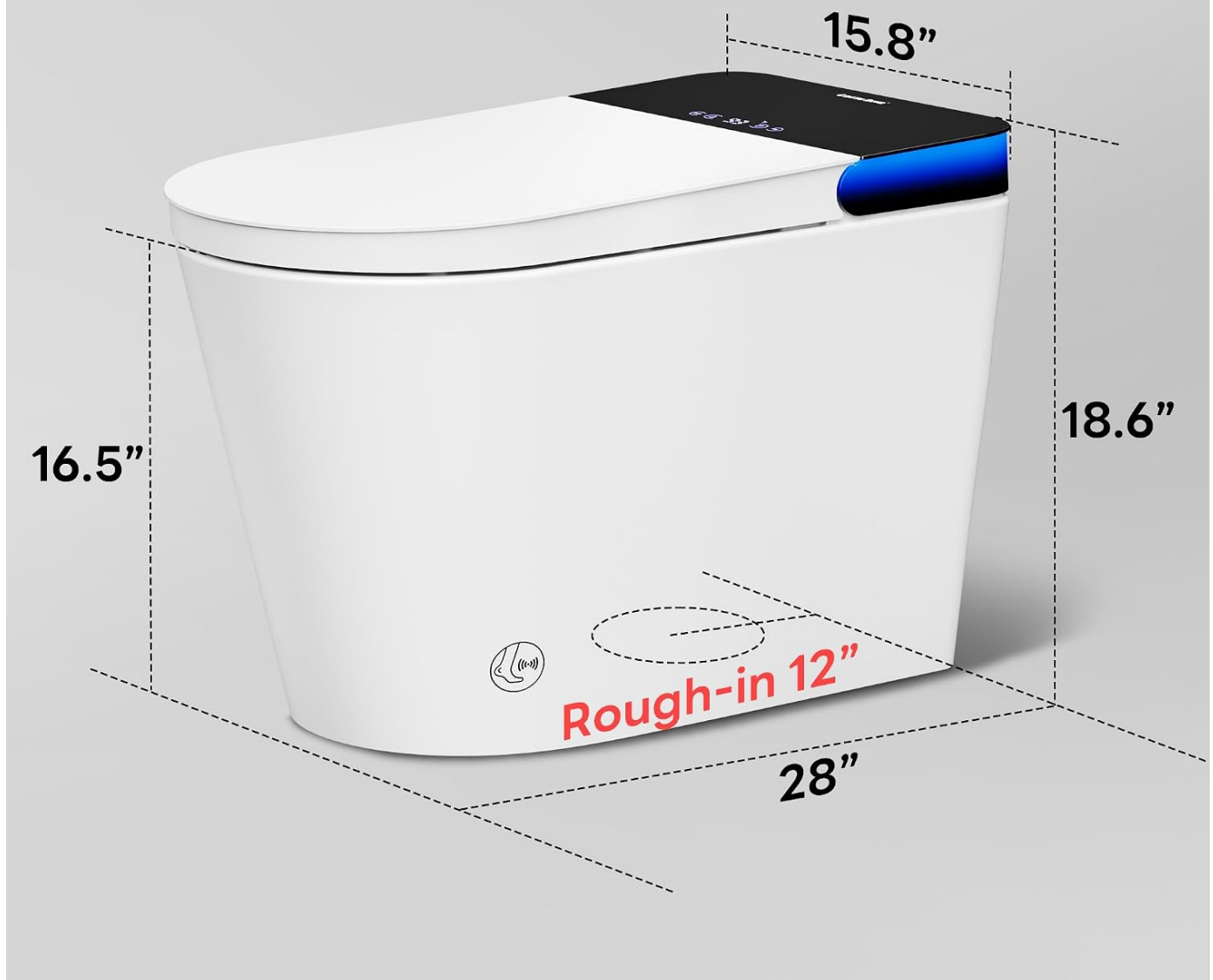
Image: ADA Comfort Height dimensions of the Casta Diva CD-U010Max Smart Toilet.
