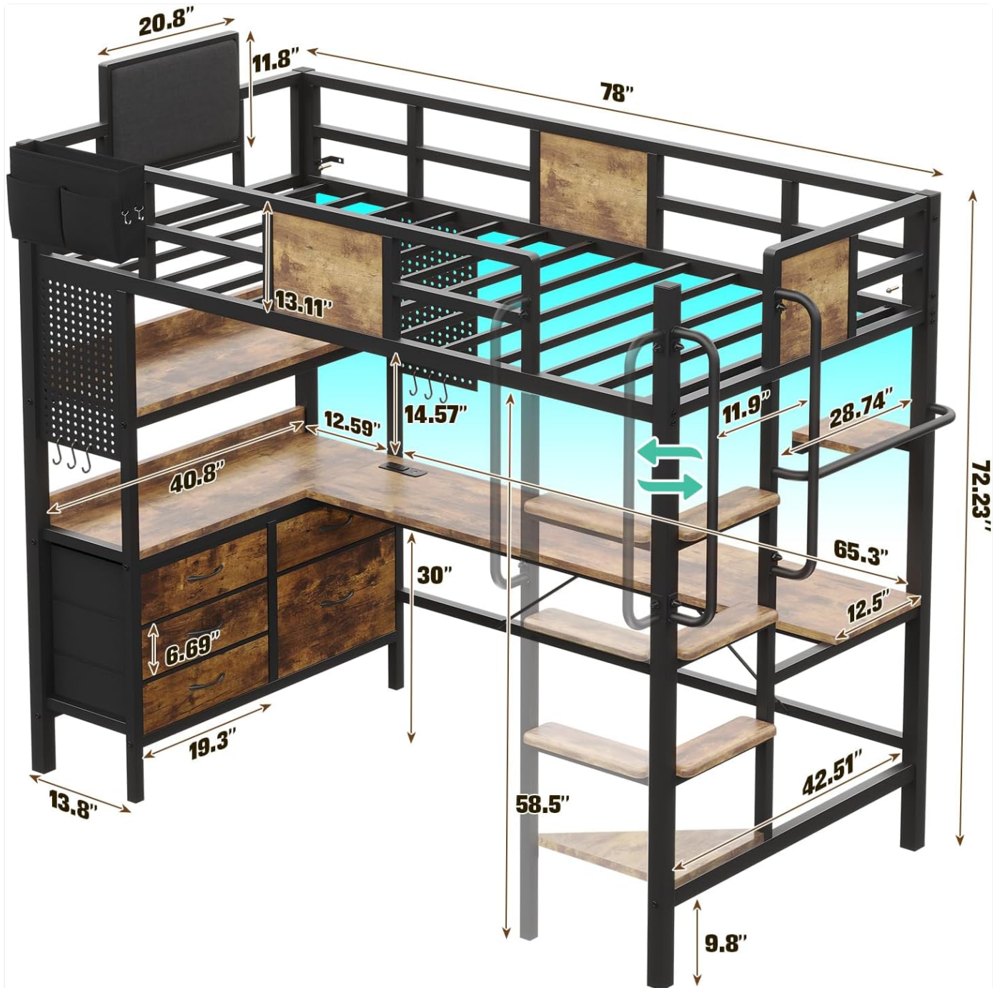
Figure 8: Product dimensions and layout.
