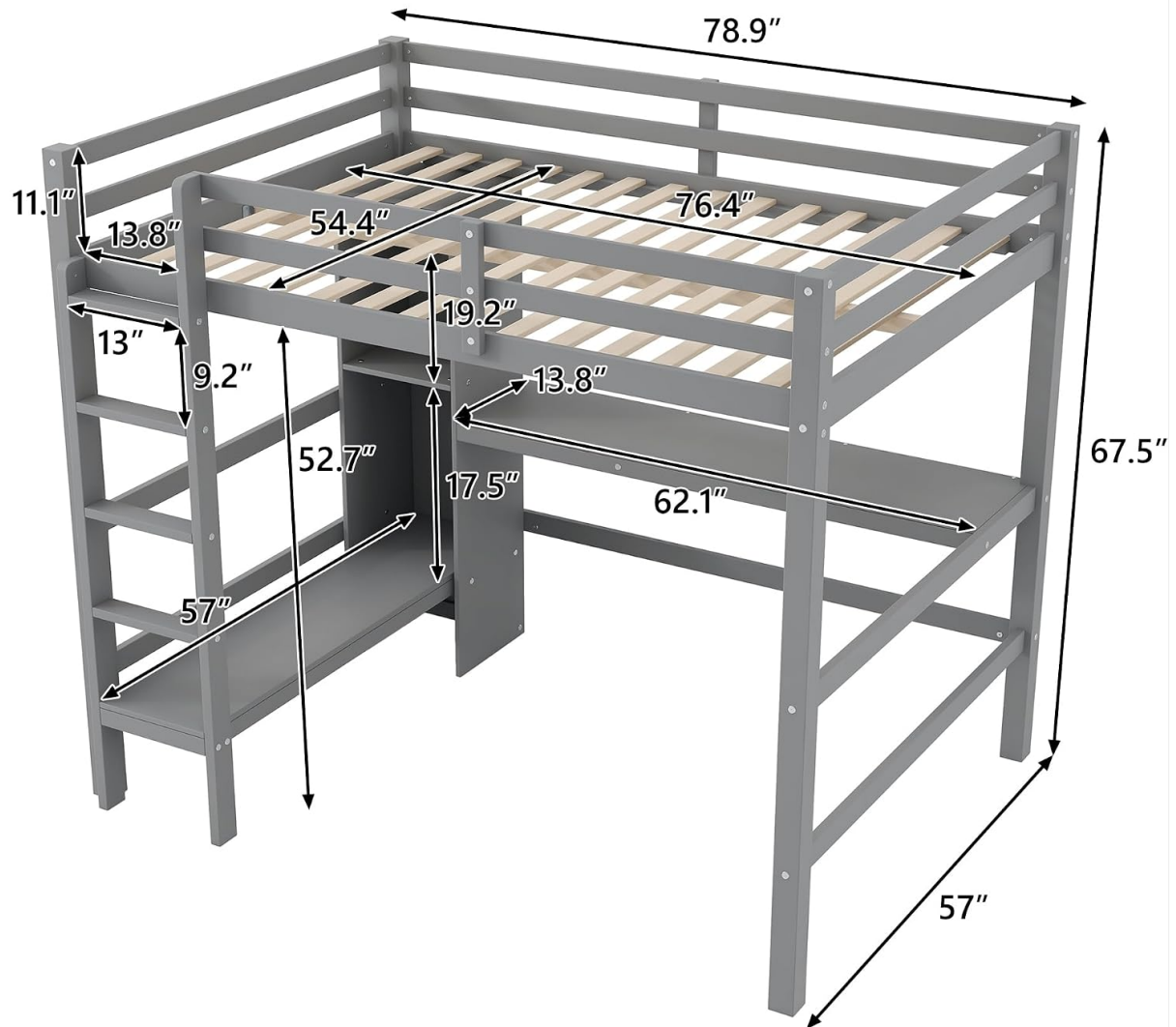
Image 4: Dimensional diagram of the SIYSNKSI Full Size Loft Bed, showing all key measurements in inches.
