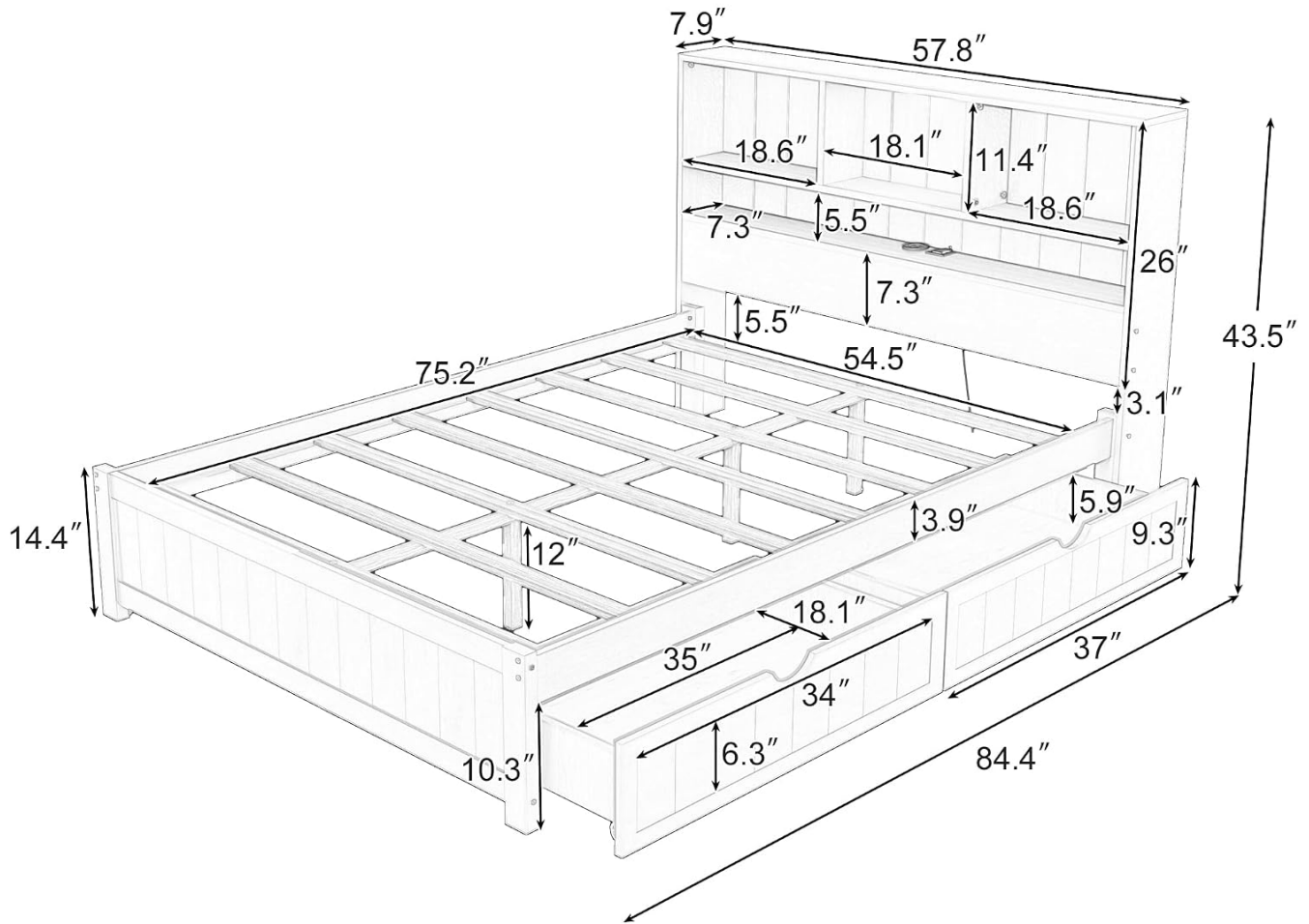
Figure 2: Detailed dimensions of the Full Size Bed Frame, including measurements for the headboard, frame length, width, and drawer sizes.
