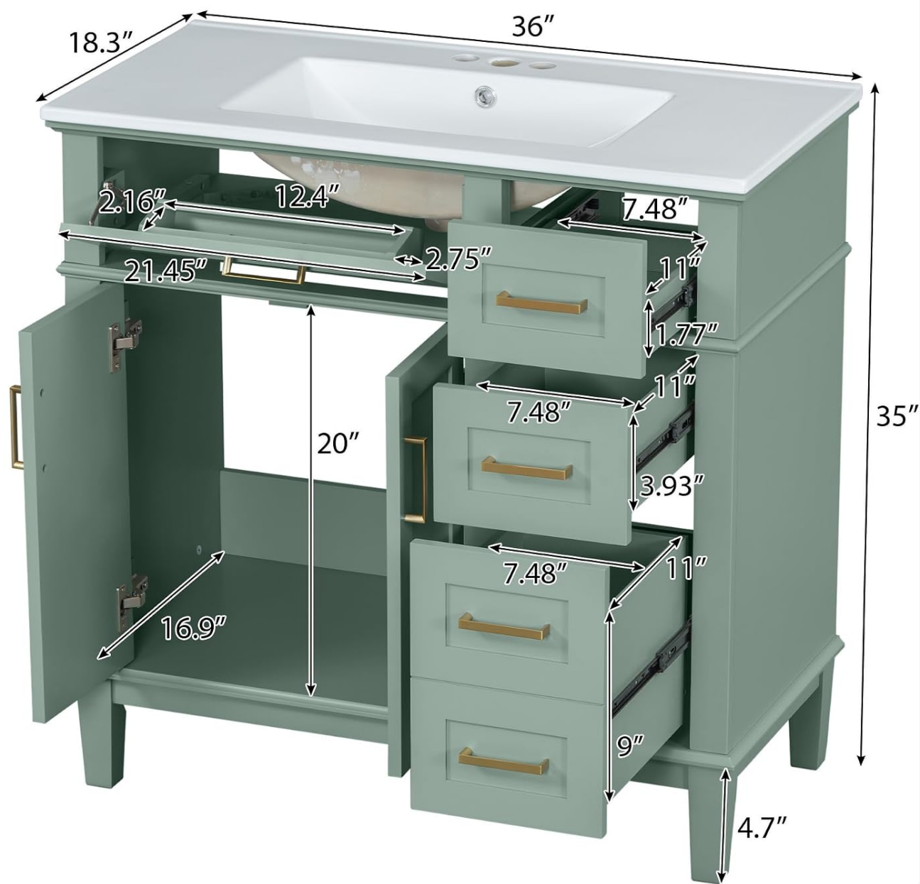
Figure 3.1: Detailed dimensions of the 36 inch bathroom vanity, including height, width, depth, and internal measurements of storage areas.
