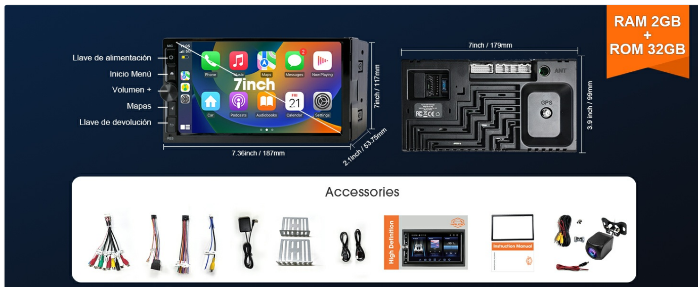
Figure 2: Detailed dimensions of the 7-inch car stereo and a visual representation of all included accessories.
