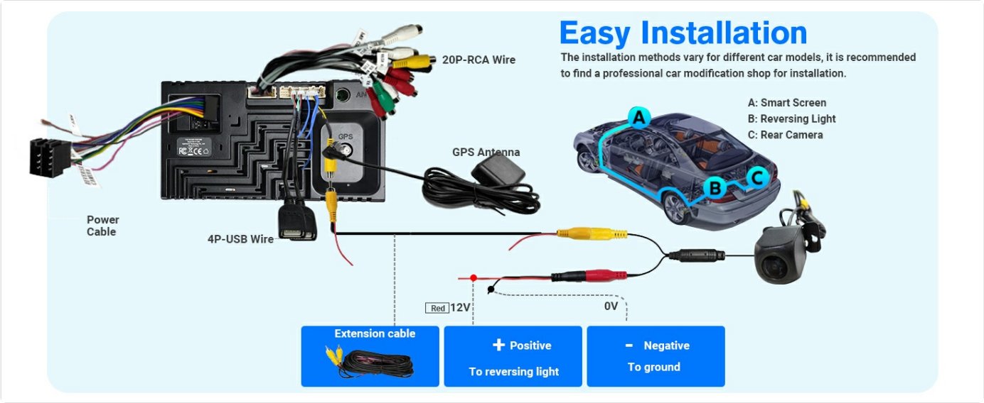
Figure 3: Easy installation wiring diagram showing connections for the smart screen, reversing light, and rear camera.
