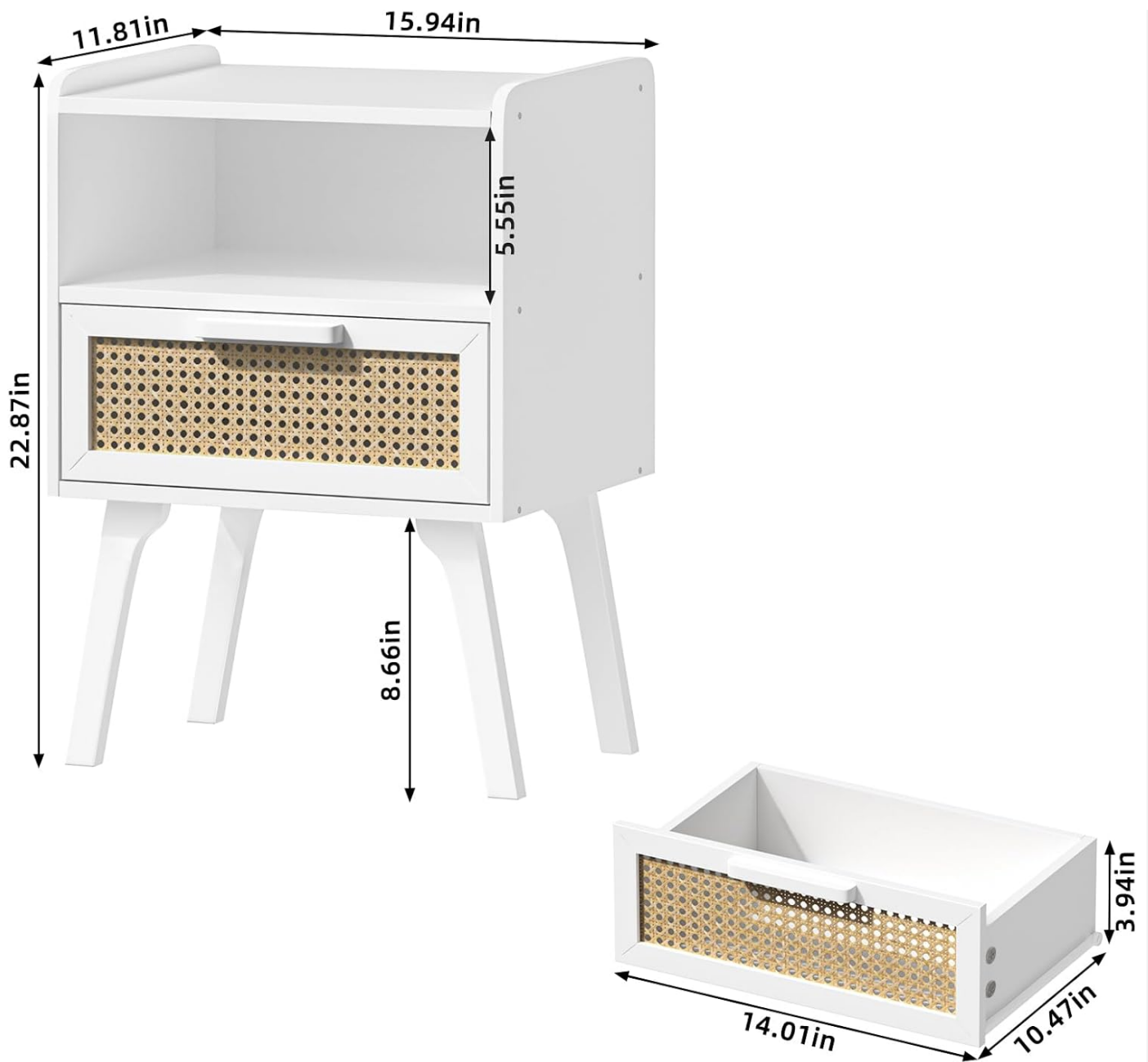
Image 7.1: Dimensional drawing of the Lerliuo Rattan Nightstand.
