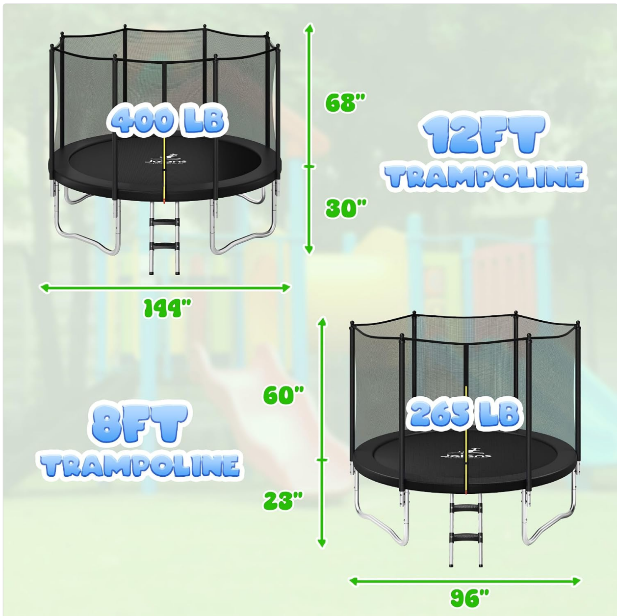
Image: Diagram illustrating the dimensions and maximum weight recommendations for different trampoline sizes.
