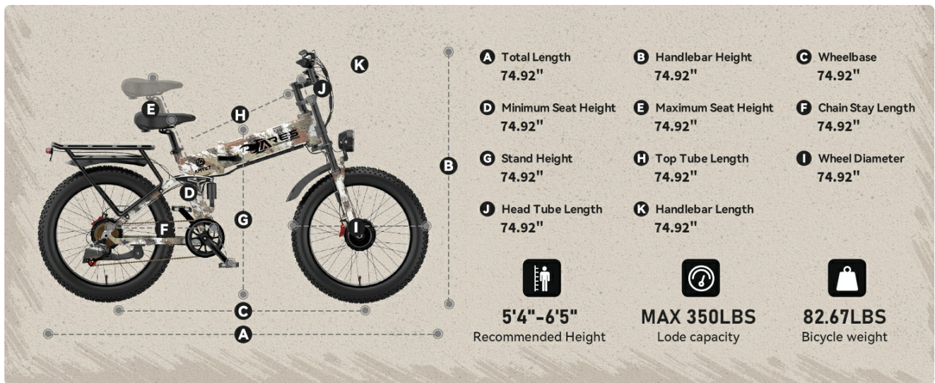
Figure 2: Detailed dimensions of the AMYET ARES E-bike for proper setup and fit.
