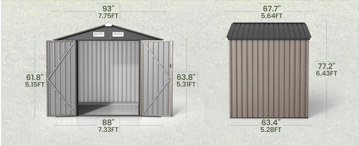
Image 1: Shed Dimensions and Installation. This image illustrates the overall dimensions of the 8x6 FT shed, including roof and base measurements, and highlights that installation requires two people for optimal ease.
