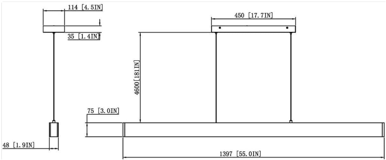
Figure 1: Dimensional drawing of the Z-Lite Hudson 1016-55L-MB-LED Linear Chandelier, illustrating overall length (55 inches), width (4.5 inches), height (3 inches), and adjustable suspension cable length (up to 181 inches).
