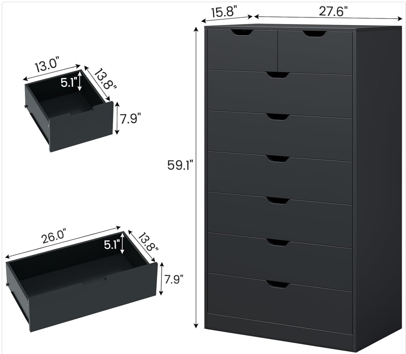
Image: Detailed dimensions of the dresser and its two types of drawers. The overall dimensions are 15.8"D x 27.6"W x 59.1"H. Small drawers are 13.0"W x 13.8"D x 7.9"H, and large drawers are 26.0"W x 13.8"D x 7.9"H.
