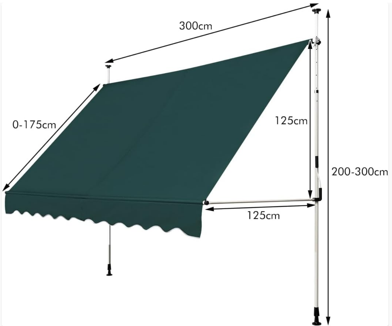
Image: Dimensional drawing of the awning, indicating a width of 300 cm, projection of 0-175 cm, and adjustable height from 200-300 cm.
