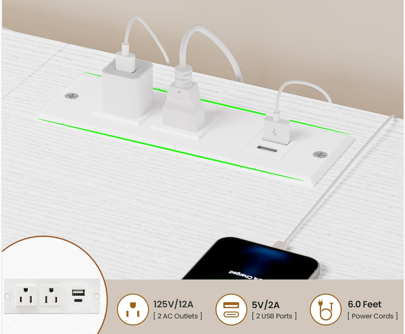
Figure 4.2: Integrated Power Outlets. This image provides a detailed view of the charging station, featuring two AC outlets and two USB ports (USB-A and Type-C) for convenient power access.
