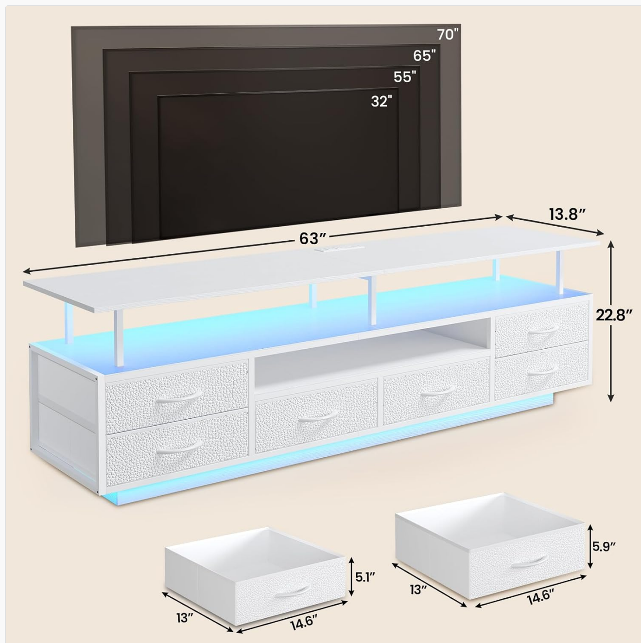
Figure 3.1: Product Dimensions and TV Compatibility. This diagram illustrates the overall dimensions of the TV stand (63" L x 13.8" W x 22.8" H) and the sizes of the fabric drawers. It also indicates compatibility with TVs ranging from 32" to 70" inches.
