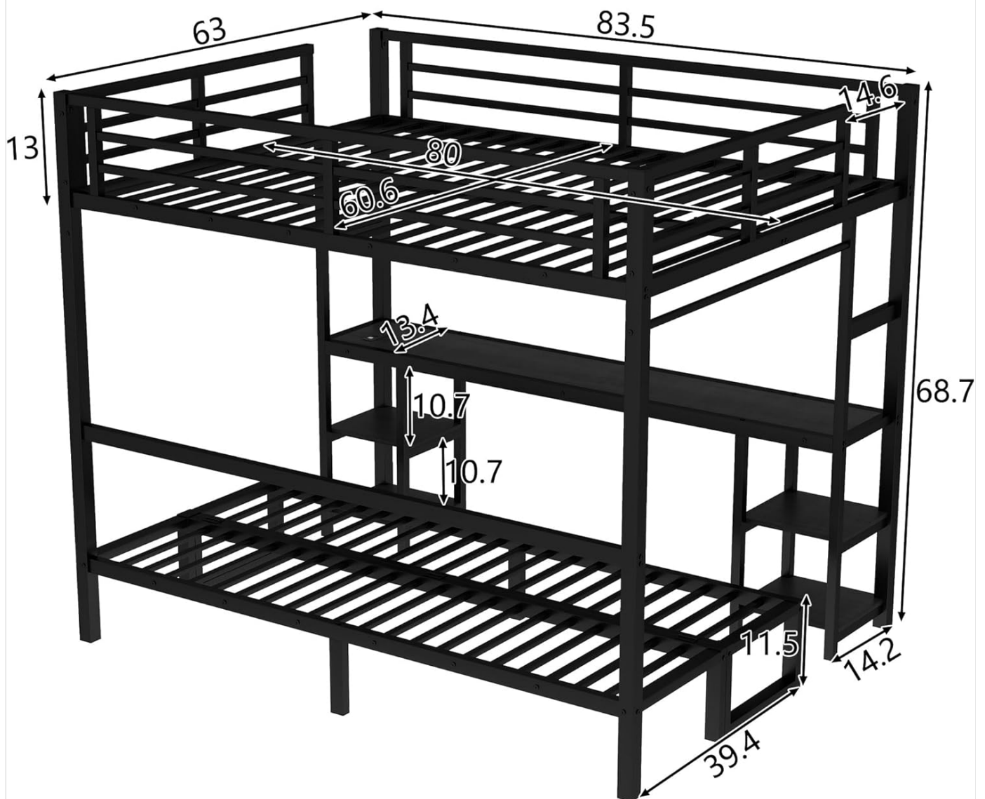
Image: A technical diagram illustrating the precise dimensions in inches of the Polibi Queen Over Twin XL Metal Bunk Bed, including height, length, and width of various sections.
