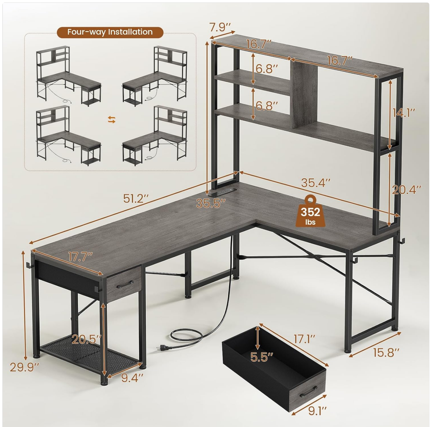
Figure 2: Desk dimensions and reversible configuration options.
