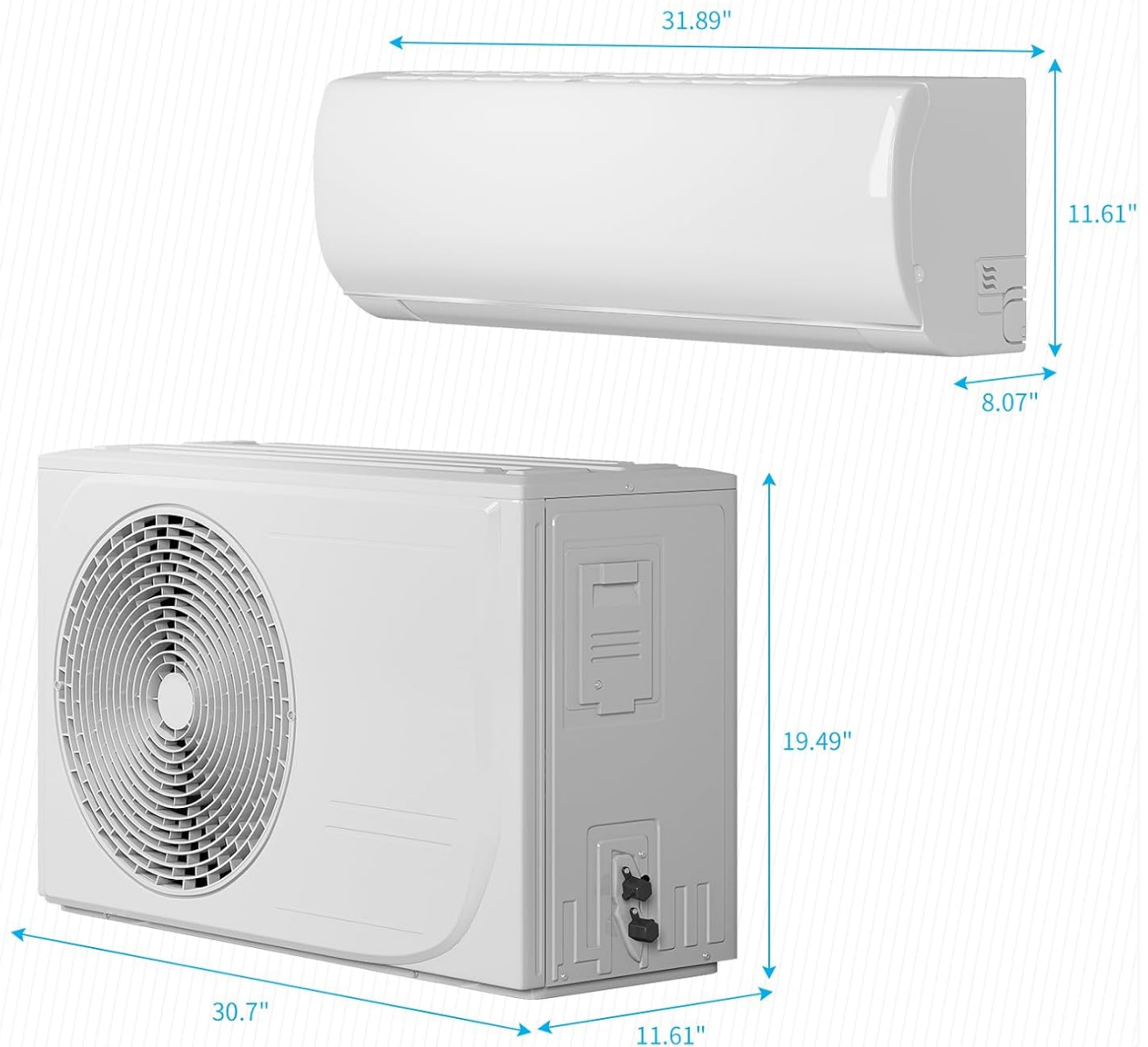
Image 4.1: Detailed dimensions for both the indoor unit (31.89" L x 11.61" H x 8.07" D) and the outdoor unit (30.7" L x 19.49" H x 11.61" D), crucial for installation planning.
