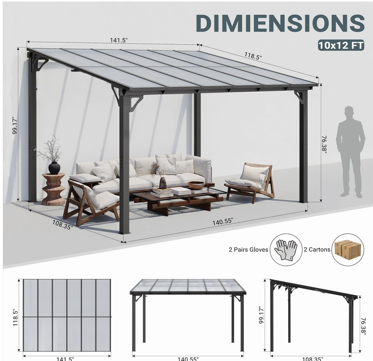
Overview of gazebo dimensions and main components.
