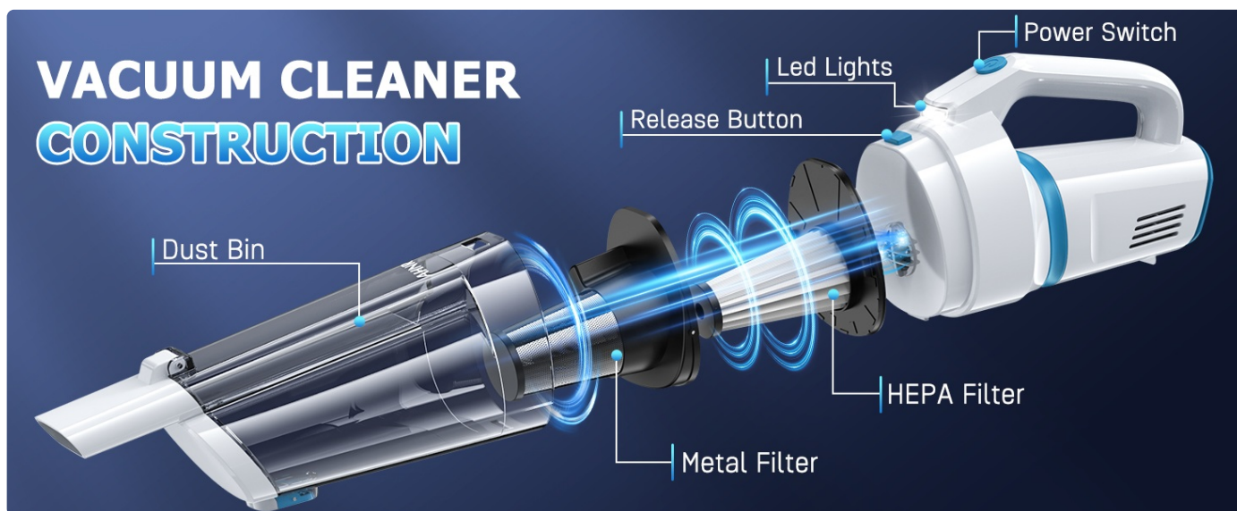
Figure 3: Vacuum Cleaner Construction Diagram.
