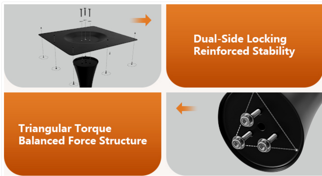
Figure 2: Assembly steps for connecting the base to the tabletop.
