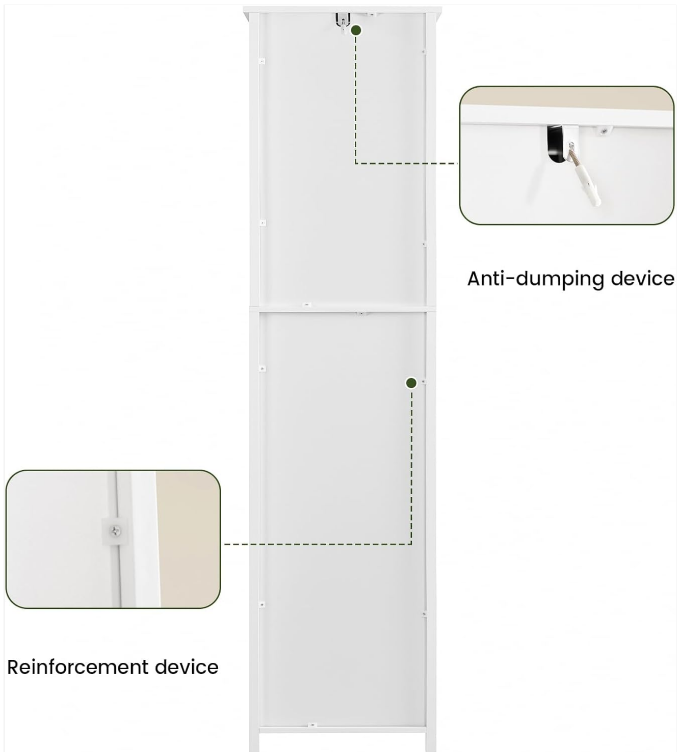
Image: Detail of the anti-tipping device and reinforcement device located on the back of the cabinet for secure installation.
