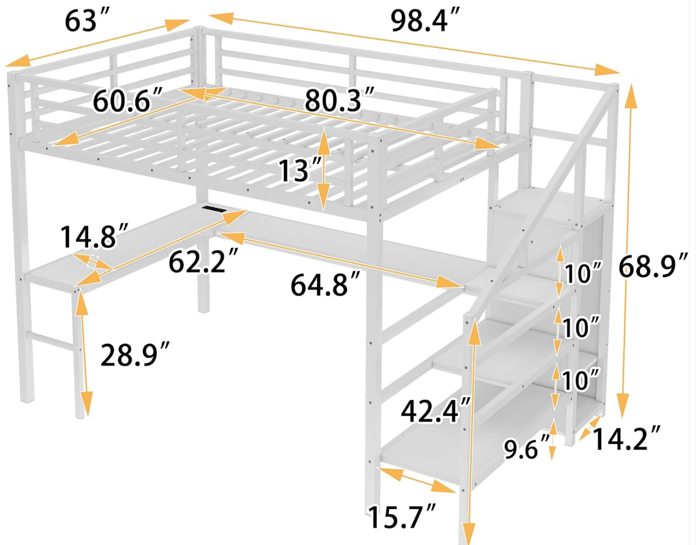
Figure 4.2: Detailed dimensions of the DERCASS Queen Metal Loft Bed, including bed frame, desk, and staircase measurements.
