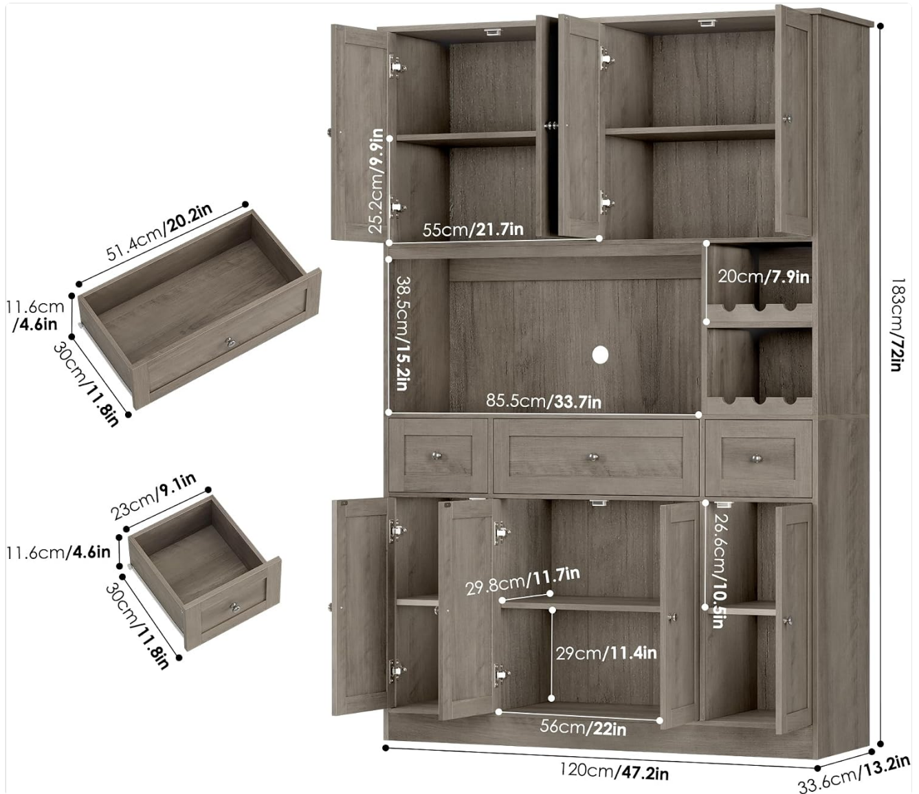
Image: Detailed diagram illustrating the dimensions of the cabinet and its various compartments, including drawers and shelves.
