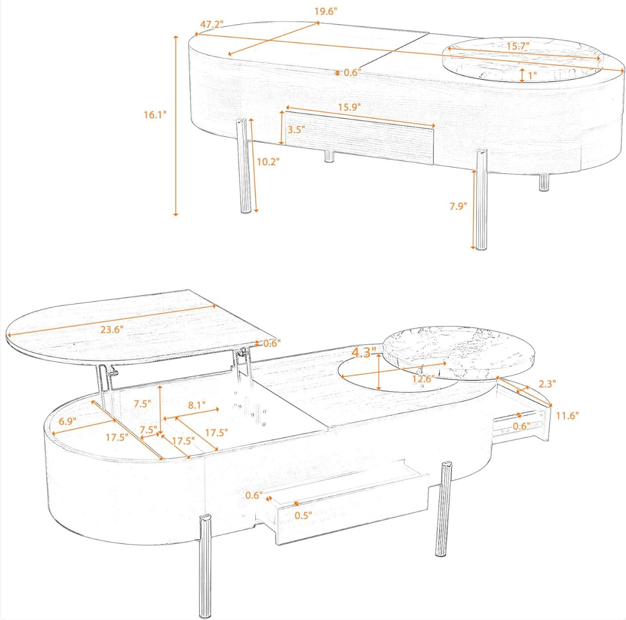
Image 3.1: Technical diagram illustrating the table's dimensions and structural elements.
