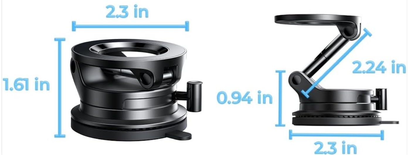
Image: Detailed dimensions and adjustable angles of the LISEN Suction Cup Phone Mount.
