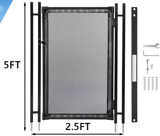
Image: An illustration detailing the gate dimensions and included hardware for the VINGLI Pool Fence Gate.
