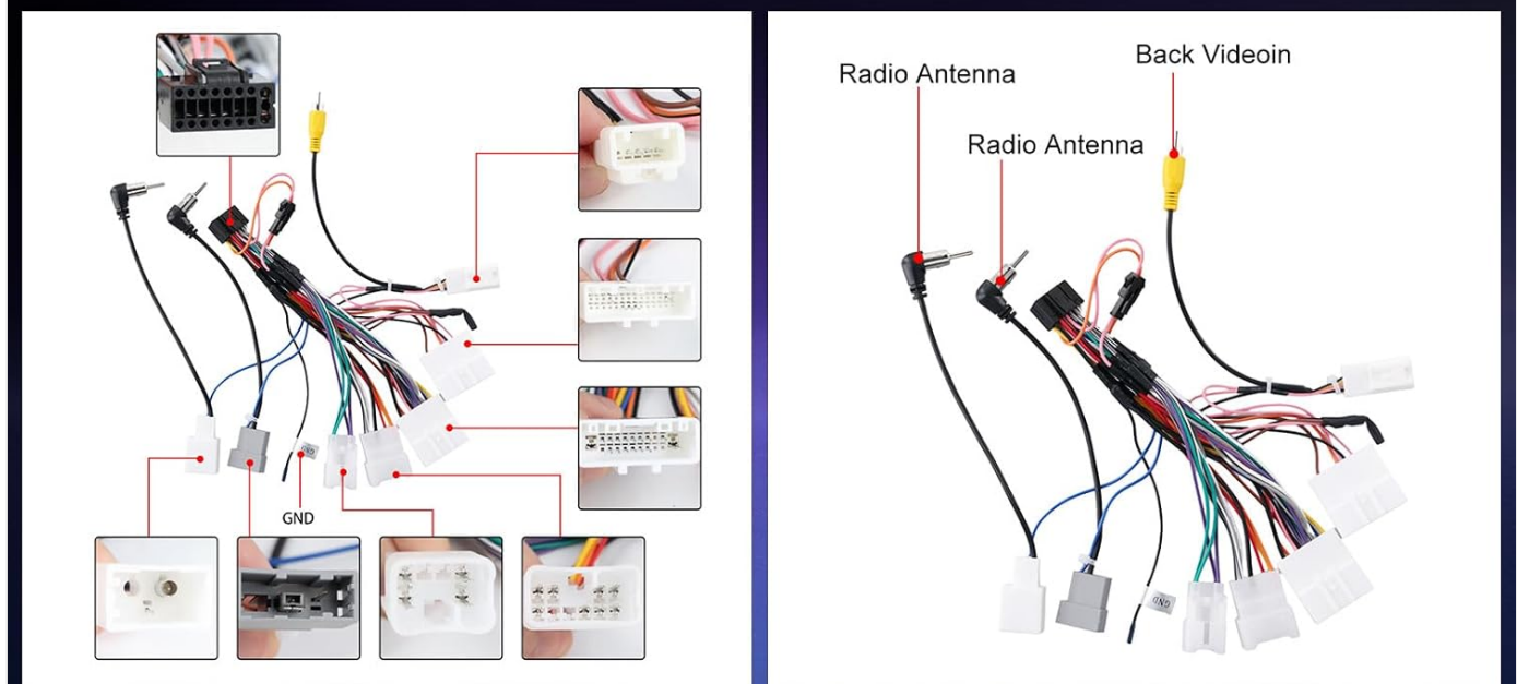
Figure 3: Connection and Wiring Diagram. This diagram provides a comprehensive overview of all necessary electrical connections for the car stereo, including power, USB, RCA, GPS antenna, reversing camera input, and radio antenna. It details the various harnesses and their corresponding functions.
