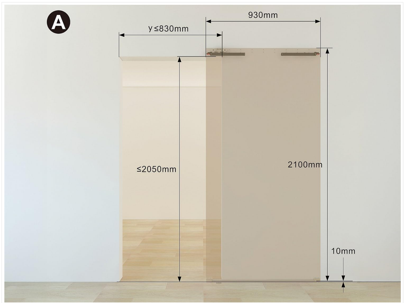
Image: Diagram A illustrates the required dimensions for the door opening and adjacent wall space for installation. Note the door width of 930mm and height of 2100mm, with a minimum clearance of 10mm from the floor.
