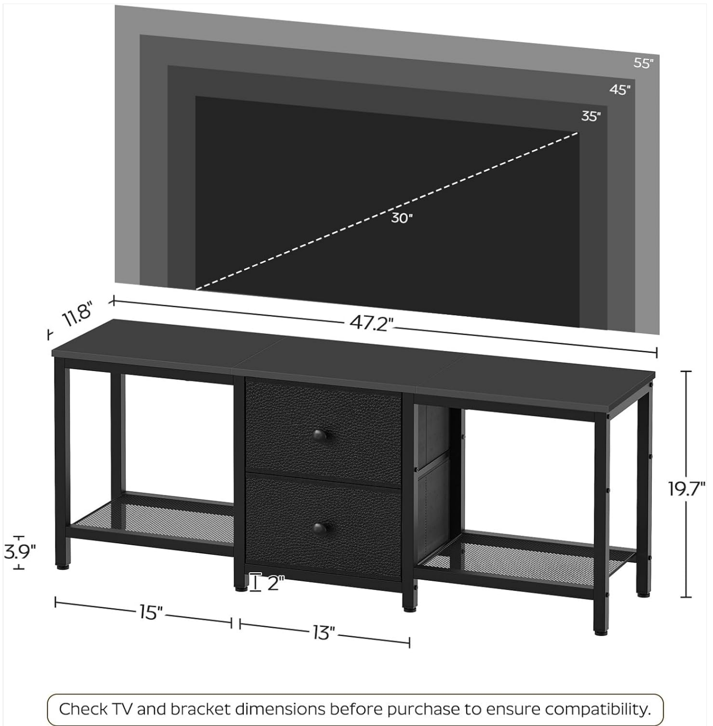
Image: Dimensional diagram of the TV stand, indicating overall length, width, and height, and the recommended TV size up to 55 inches.
