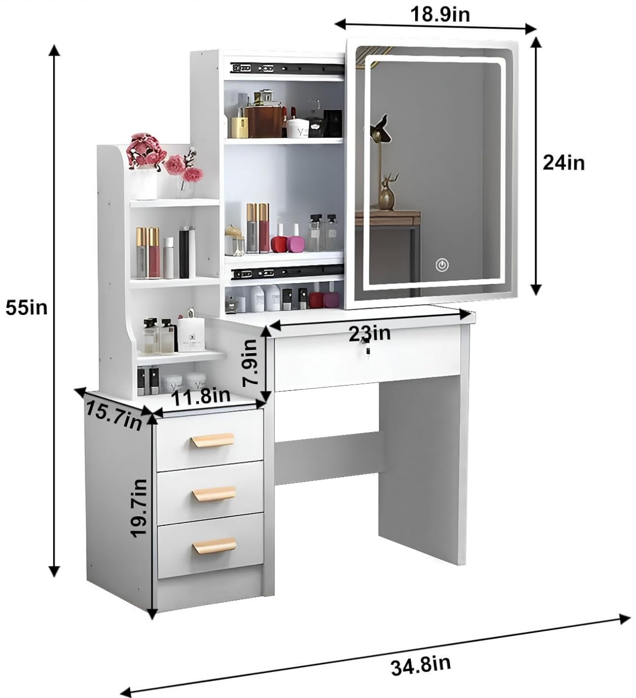
Figure 5: Detailed product dimensions.
