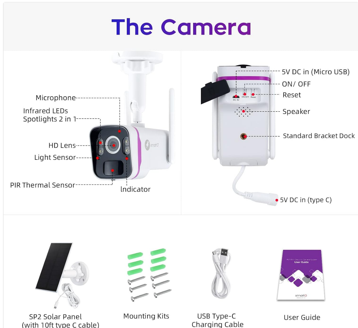
Image: Detailed diagram of the xmartO BC4-SP camera components.
