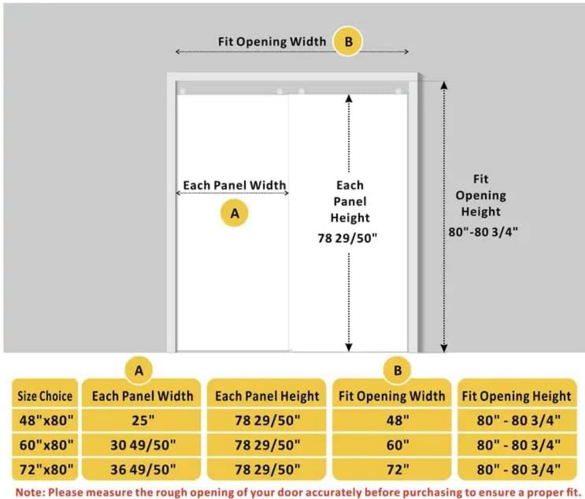
Figure 1: Standard Sliding Door Dimensions. This diagram illustrates the panel width and height, and the corresponding fit opening width and height for various door sizes, including the 60"x80" model.
