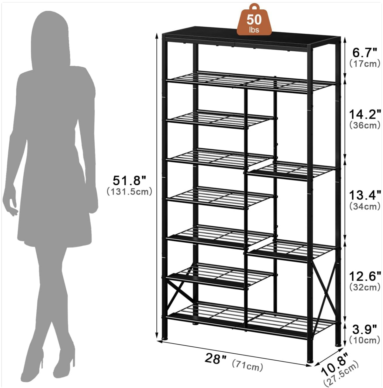
Image 7.1: Product dimensions.
