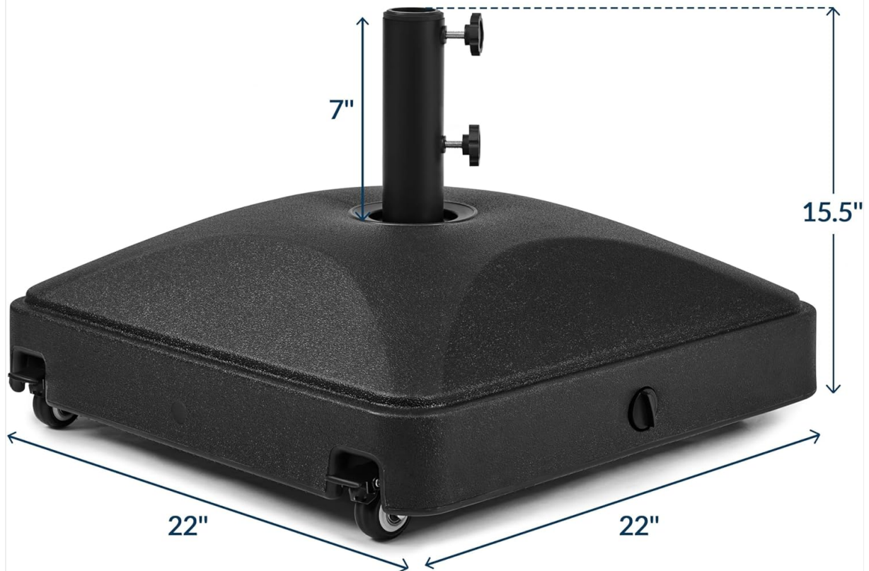
Image: Diagram illustrating the product dimensions: 22 inches by 22 inches base, and 15.5 inches total height with a 7-inch pole holder.
